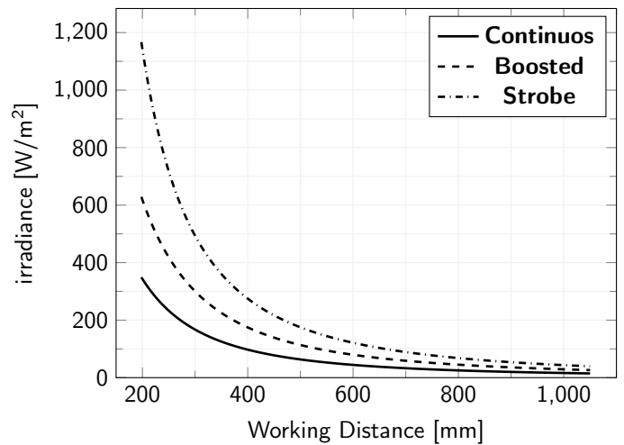
Irradiance Characteristics
